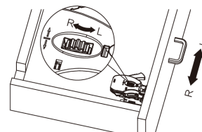
Side adjustment ± 1.5mm
